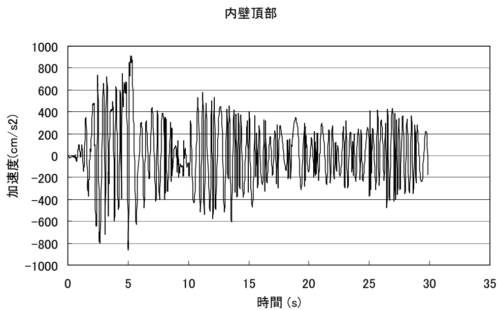
Figure 3.11 Time History of Horizontal Acceleration at the Top of the Partition Wall (Maximum Acceleration = 883 gal at t = 5.31 s)
